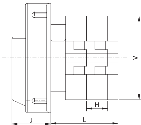
S 100, 160 JU
